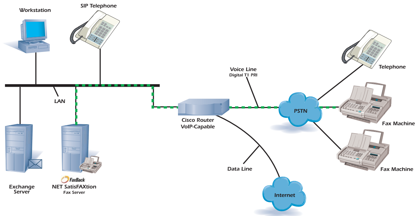
Figure 2 Boardless VoIP Fax Server
